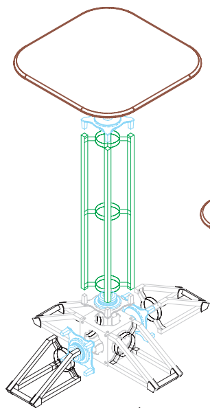
Racetrack Parts exploded
